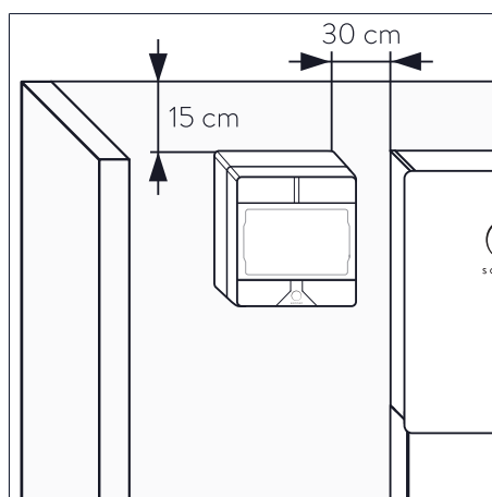
Illustration 2: Minimum distances
